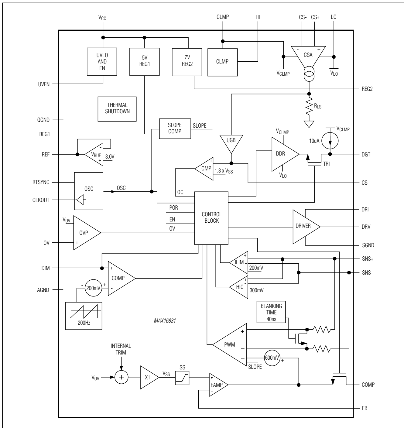
Functional Diagram
